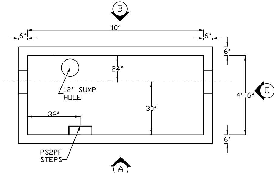
PLAN-STRUCTURE
